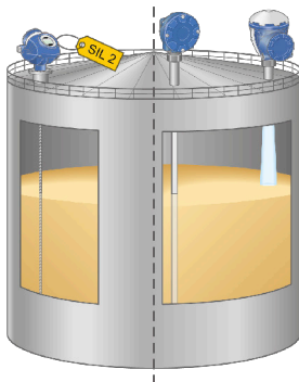
Fixed Roof
