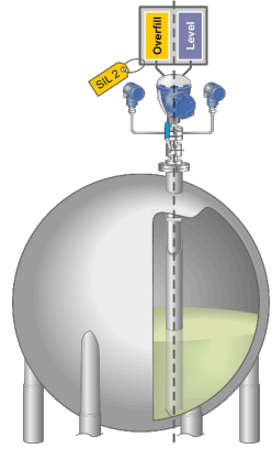
Sphere
