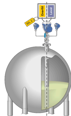
FMCW Radar 2-in-1
