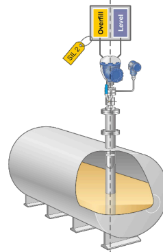
FMCW Radar 2-in-1
