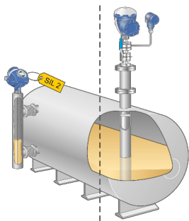
2-wire Guided Wave Radar (5300)
