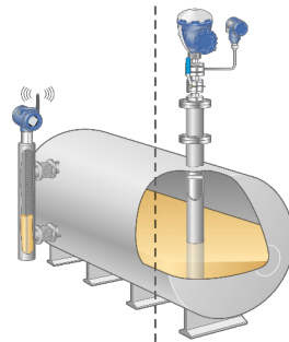
Wireless Guided Wave Radar (3308)
